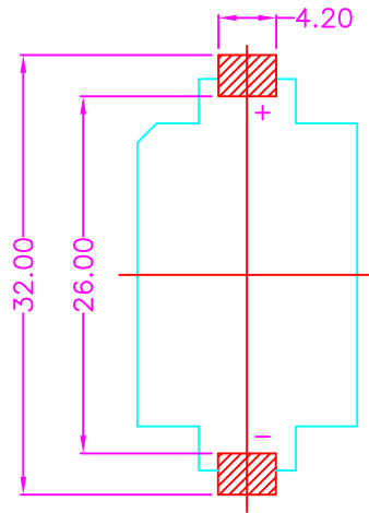
P.C.B. LAYOUT TOP VIEW ±0.05
