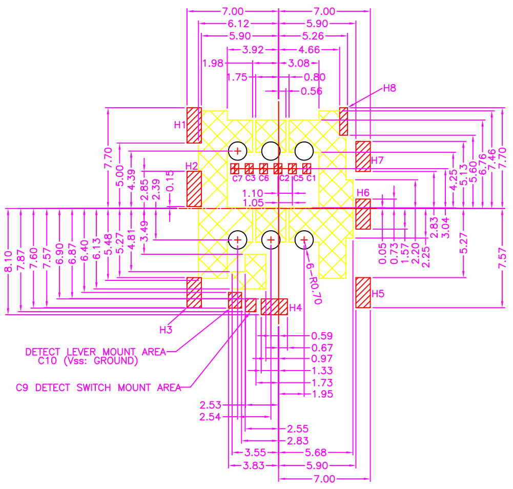
P.C.B. LAYOUT TOP VIEW ±0.05
