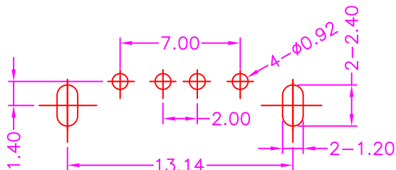
P.C.B LAYOUT TOP VIEW ±0.05
