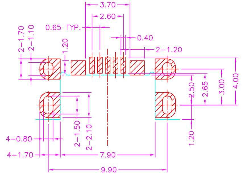
P.C.B. LAYOUT TOP VIEW ±0.05
