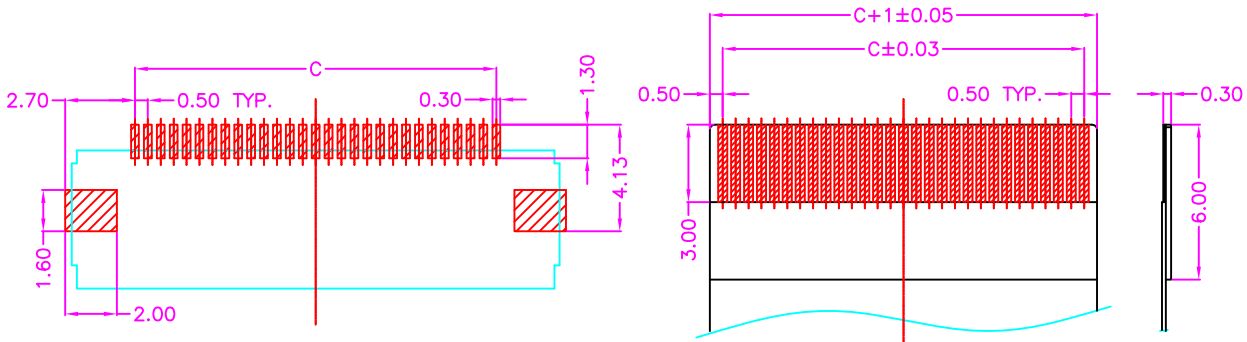
P.C.B LAYOUT TOP VIEW ±0.05
