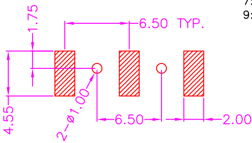
P.C.B LAYOUT TOP VIEW ±0.05
