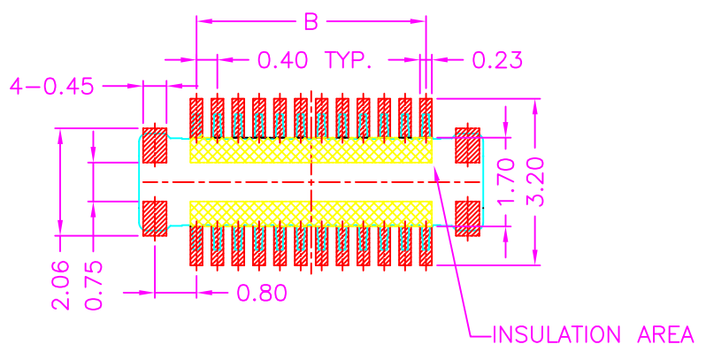
P.C.B LAYOUT TOP VIEW ±0.05
