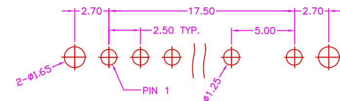
P.C.B. LAYOUT TOP VIEW ±0.05
