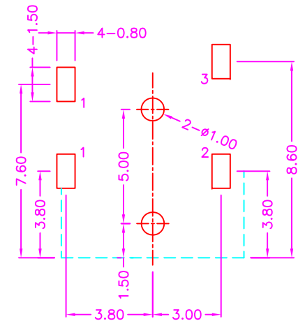
P.C.B LAYOUT TOP VIEW ±0.05
