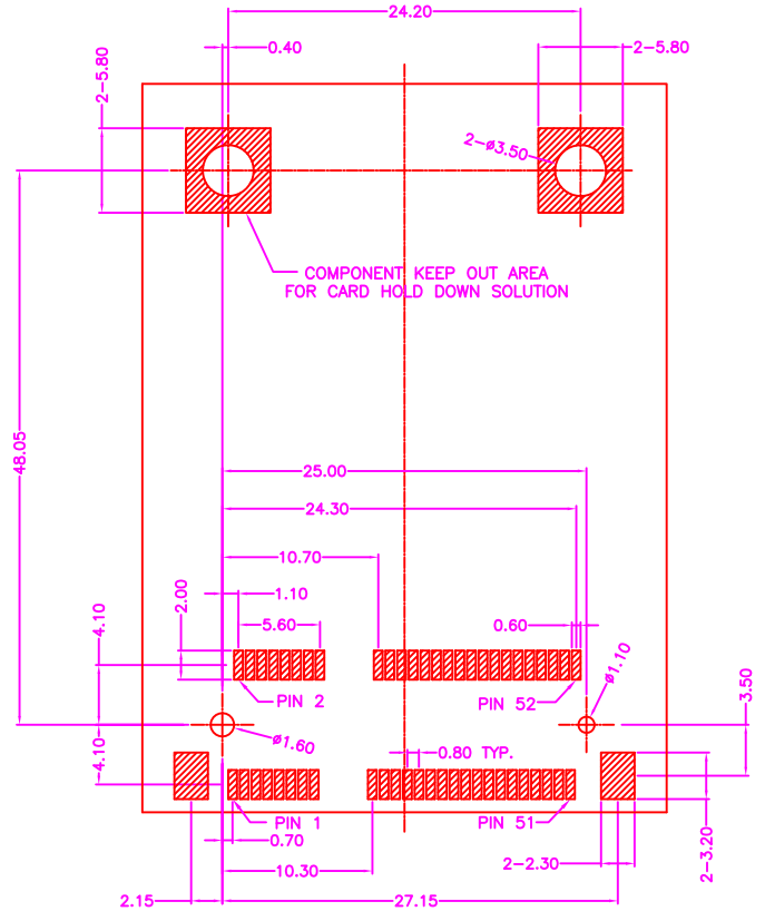
P.C.B LAYOUT TOP VIEW ±0.05
