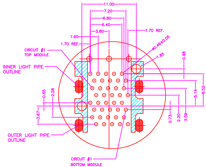
P.C.B. LAYOUT TOP VIEW ±0.05 DEATIL A SCALE 2:1
