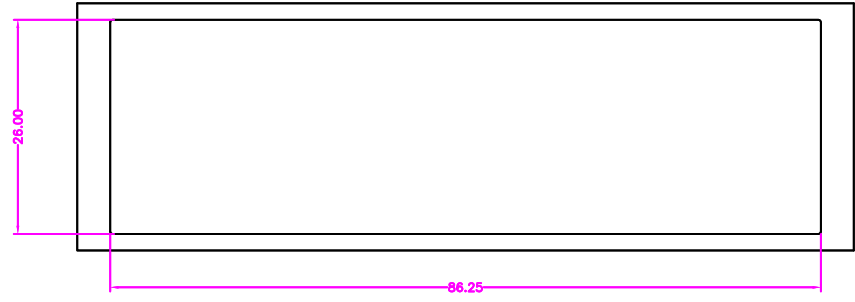
BEZEL CUT-OUT CENTER SPACING DETAIL BEZEL THICKNESS:0.8-2.6
