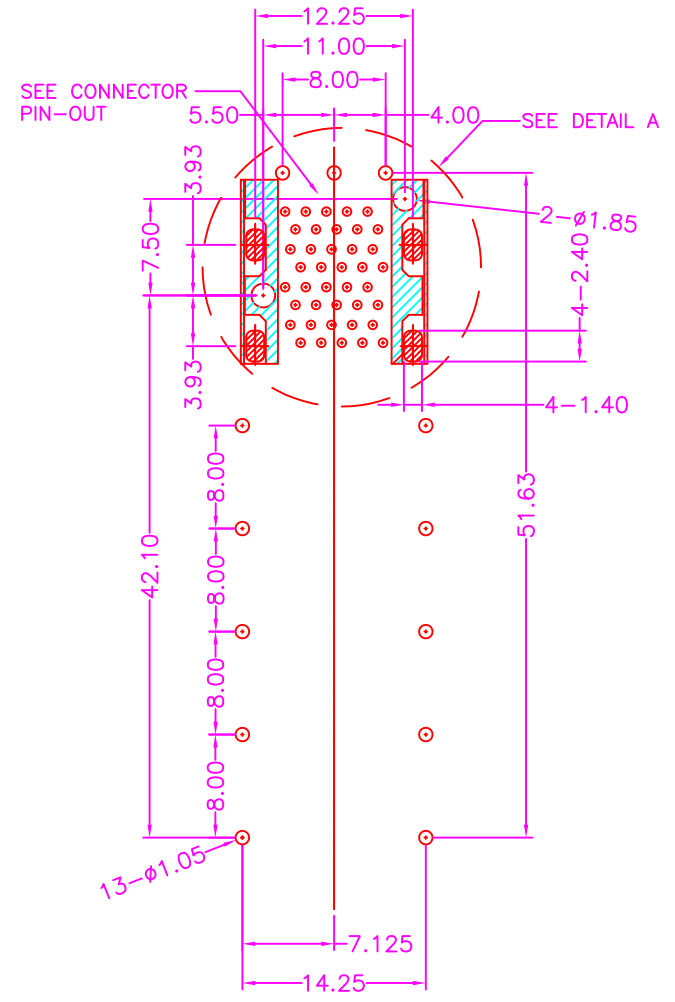
P.C.B. LAYOUT TOP VIEW \pm 0.05
