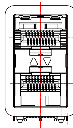
021BP-0*C-13 WITH INNER LIGHT PIPES
