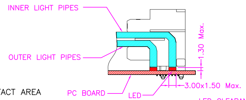
LED CLEARANCE REQUIREMENTS
