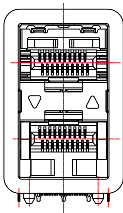
021BP-0*C-12 WITH OUTER LIGHT PIPES
