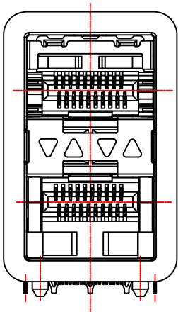
021BP-0*C-11 WITH INNER & OUTER LIGHT PIPES
