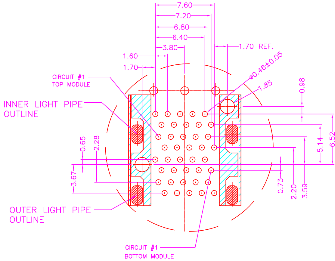
P.C.B. LAYOUT TOP VIEW \pm 0.05
