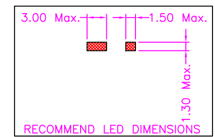
LED CLEARANCE REQUIREMENTS
