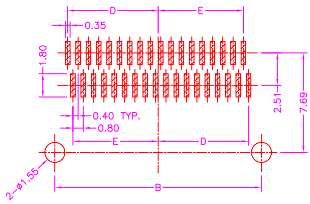
P.C.B LAYOUT TOP VIEW ±0.05
