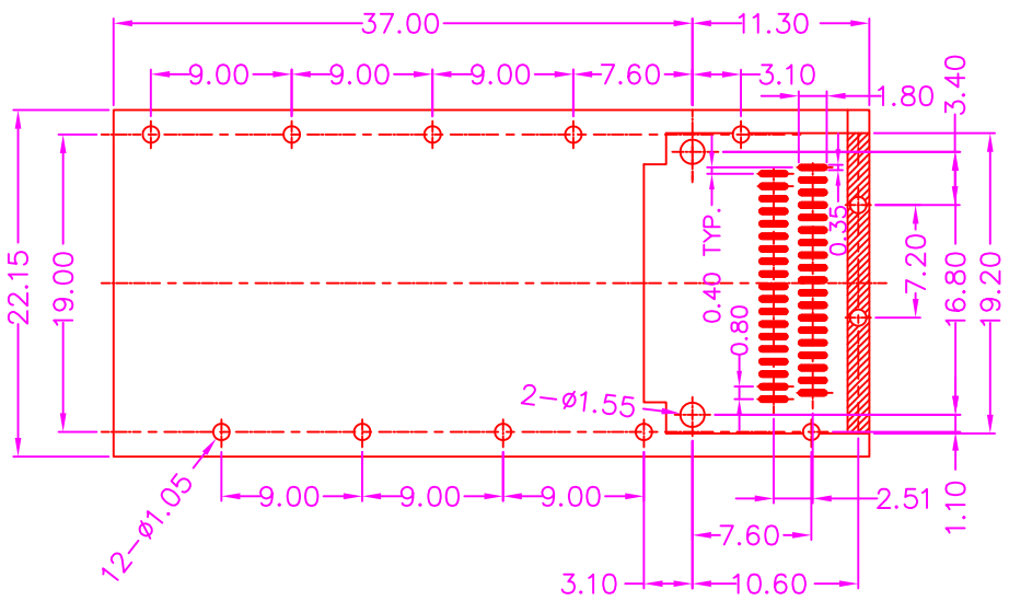
P.C.B LAYOUT TOP VIEW ±0.05
