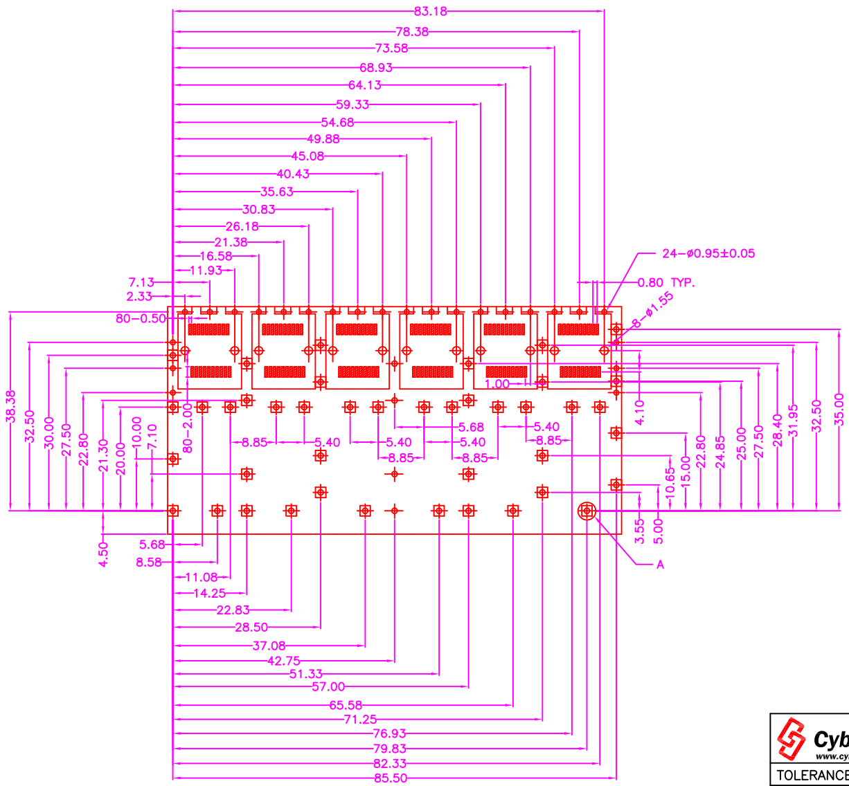
P.C.B. LAYOUT TOP VIEW ±0.05
