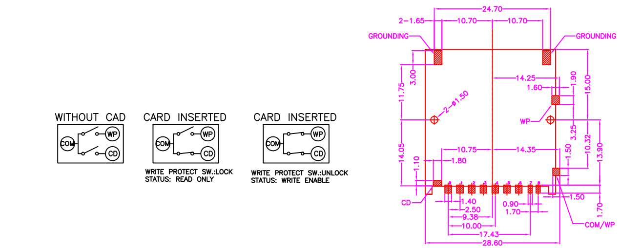
P.C.B. LAYOUT TOP VIEW ±0.05
