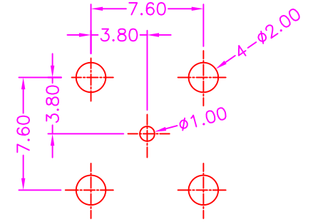
P.C.B LAYOUT TOP VIEW ±0.05
