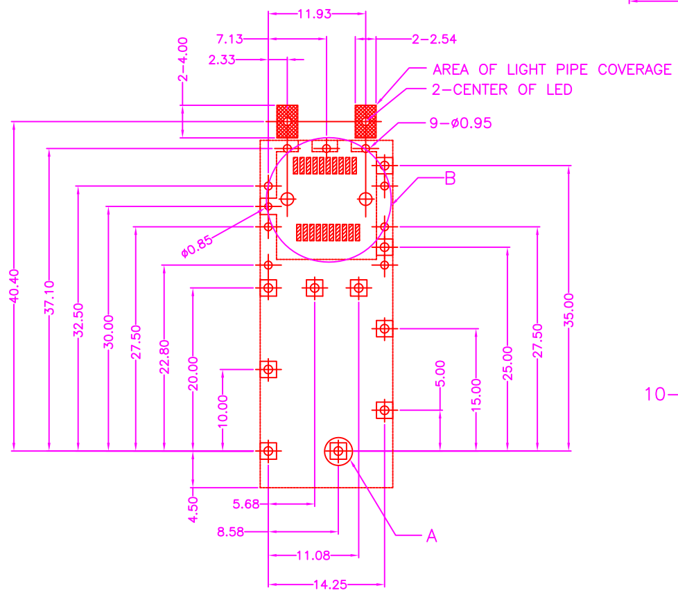
P.C.B LAYOUT TOP VIEW ±0.05
