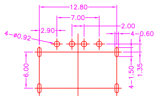
P.C.B. LAYOUT TOP VIEW ±0.05
