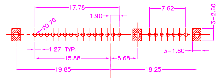
P.C.B LAYOUT TOP VIEW ±0.05
