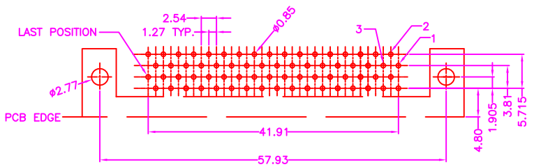
P.C.B LAYOUT TOP VIEW ±0.05
