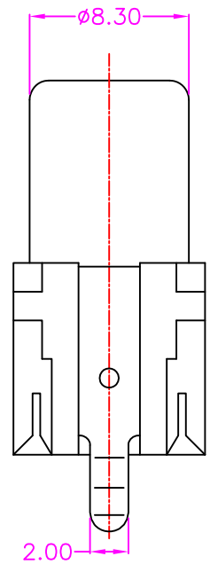
P.C.B LAYOUT TOP VIEW ±0.05
