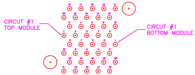
CONNECTOR PIN-OUT COMPONENT SIDE OF BOARD
