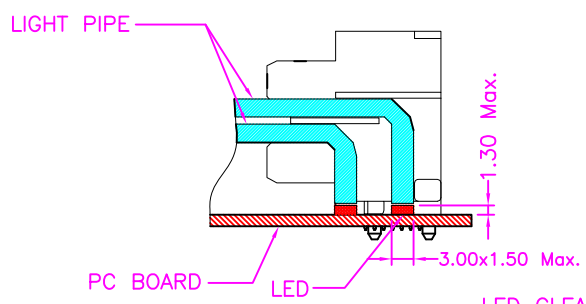
LED CLEARANCE REQUIREMENTS
