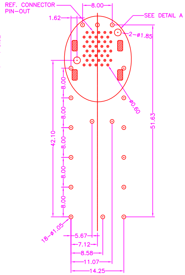
P.C.B LAYOUT TOP VIEW ±0.05
