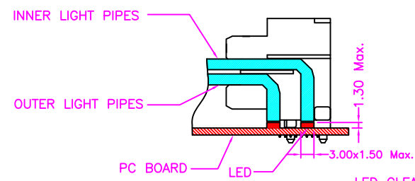
LED CLEARANCE REQUIREMENTS
