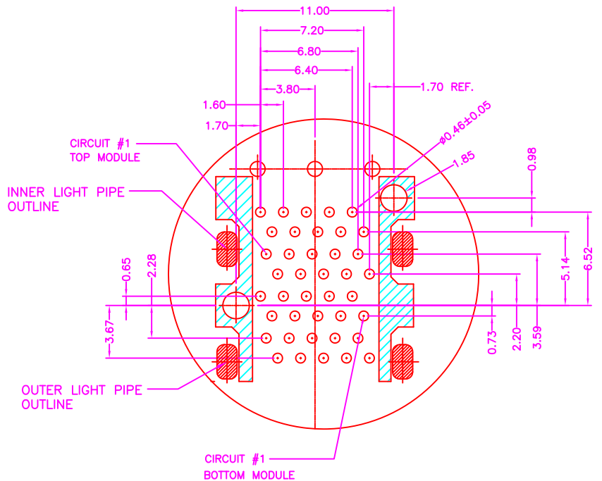
P.C.B. LAYOUT TOP VIEW ±0.05
