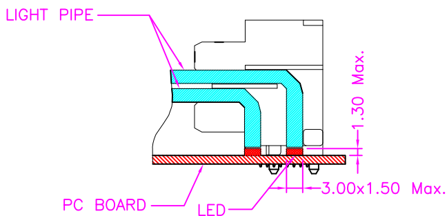
LED CLEARANCE REQUIREMENTS
