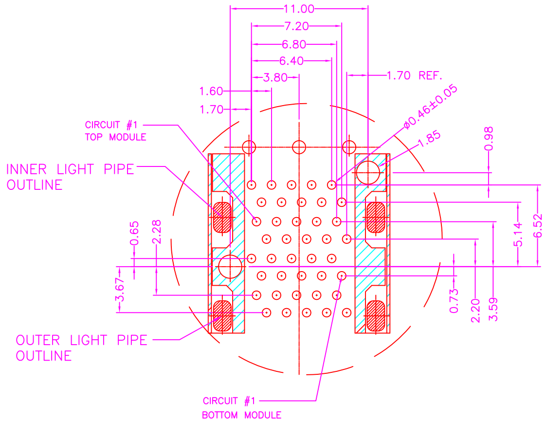
P.C.B LAYOUT TOP VIEW ±0.05
