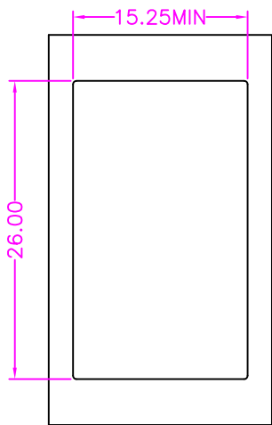
BEZEL CUT-OUT CENTER SPACING DETAIL BEZEL THICKNESS:0.8-2.6
