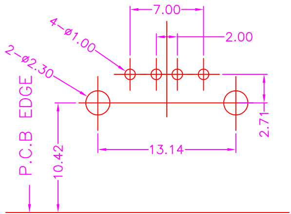
P.C.B LAYOUT TOP VIEW ±0.05
