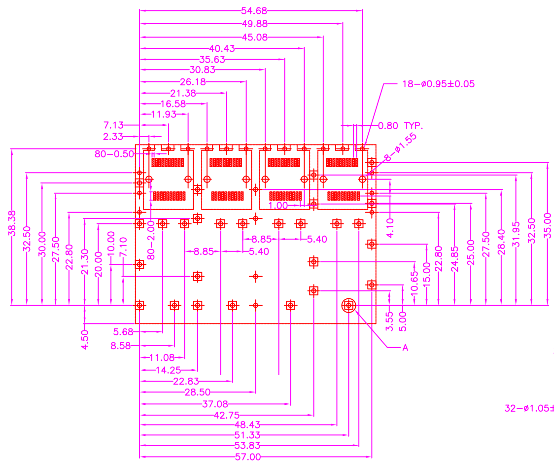
P.C.B. LAYOUT TOP VIEW ±0.05
