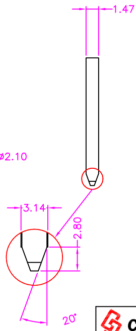
SECONDARY (SOLDER) SIDE
