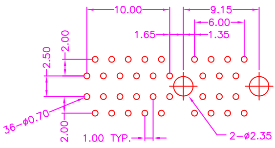
P.C.B. LAYOUT TOP VIEW ±0.05
