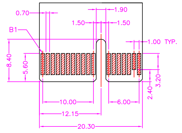
PRIMARY (COMPONENT) SIDE
