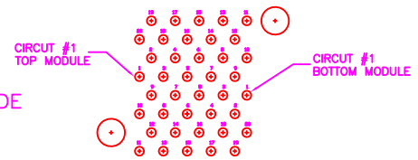
CONNECTOR PIN-OUT COMPONENT SIDE OF BOARD
