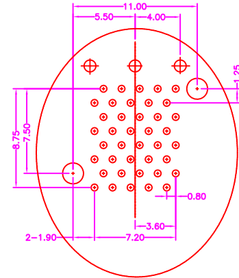
DEATIL A SCALE 2:1
