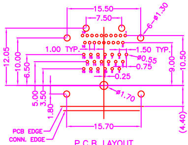
P.C.B LAYOUT TOP VIEW ±0.05
