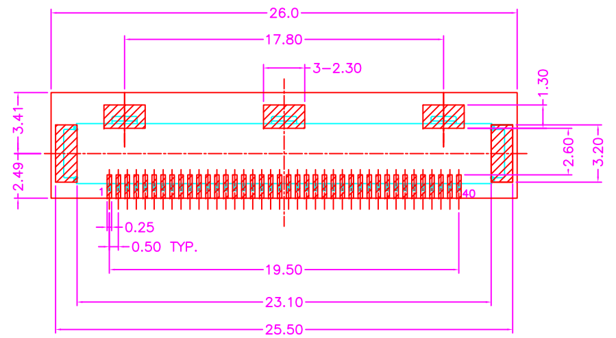
P.C.B. LAYOUT TOP VIEW ±0.05
