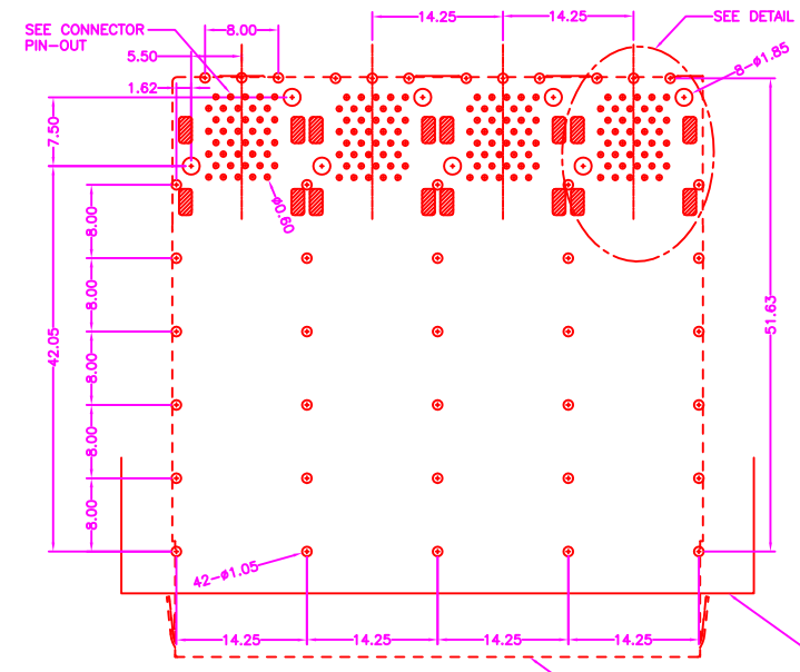
P.C.B. LAYOUT TOP VIEW ±0.05
