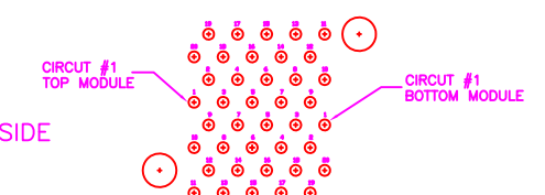
CONNECTOR PIN-OUT COMPONENT SIDE OF BOARD
