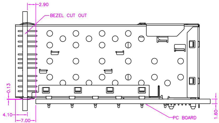
BEZEL CUT-OUT CENTER SPACING DETAIL BEZEL THICKNESS:0.8-2.6
