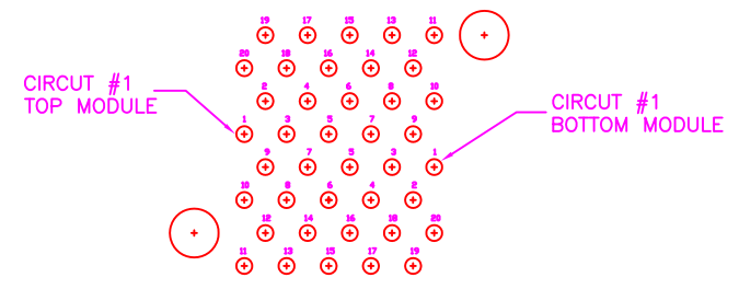
CONNECTOR PIN-OUT COMPONENT SIDE OF BOARD
