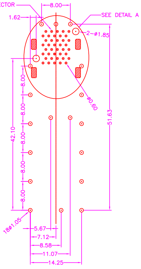
P.C.B LAYOUT TOP VIEW ±0.05
